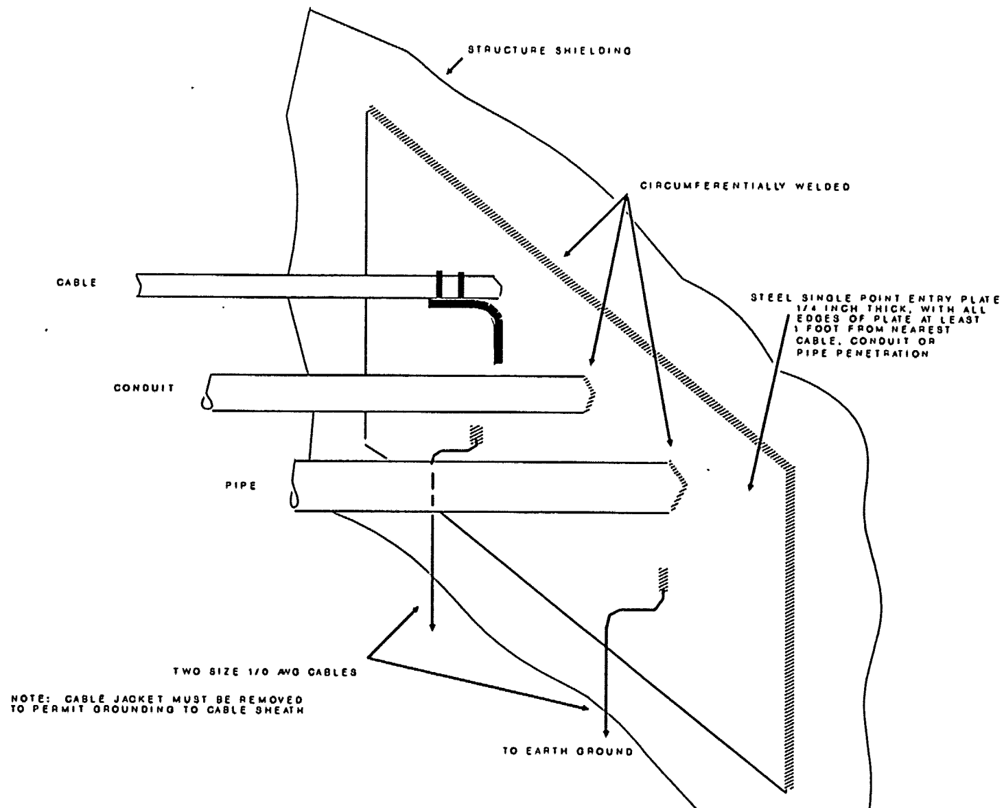
Figure 4. Typical Entry Plate Showing Rigid Cable, Conduit, and Pipe Penetrations
